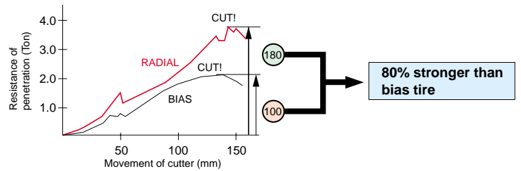
Force needed for object to penetrate the tire
